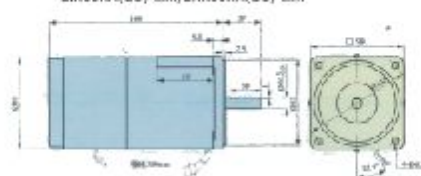
马达MOTOR 2IK60RA(GU)-□M/2RK60RA(GU)-□M
