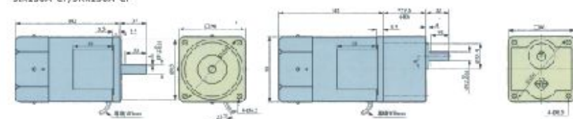
马达MOTOR 5IK90A(GN)-□F/5RK90A(GN)-□F 5IK120A(GN)-□F/5RK120A(GN)-□F 5IK150A(GN)-□F/5RK150A(GN)-□F
