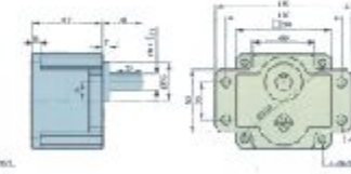
5GUU 方键: 5X5X25
