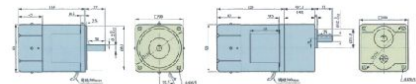
马达MOTOR 5IK60A(GN)-□F/5RK60A(GN)-□F
