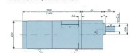
马达MOTOR 5IK60RGU-□M/SRK60RGU-□M 5IK90RGU-□M/SRK90RGU-□M 5IK120RGU-□M/SRK120RGU-□M 5IK150RGU-□M/SRK150RGU-□M
